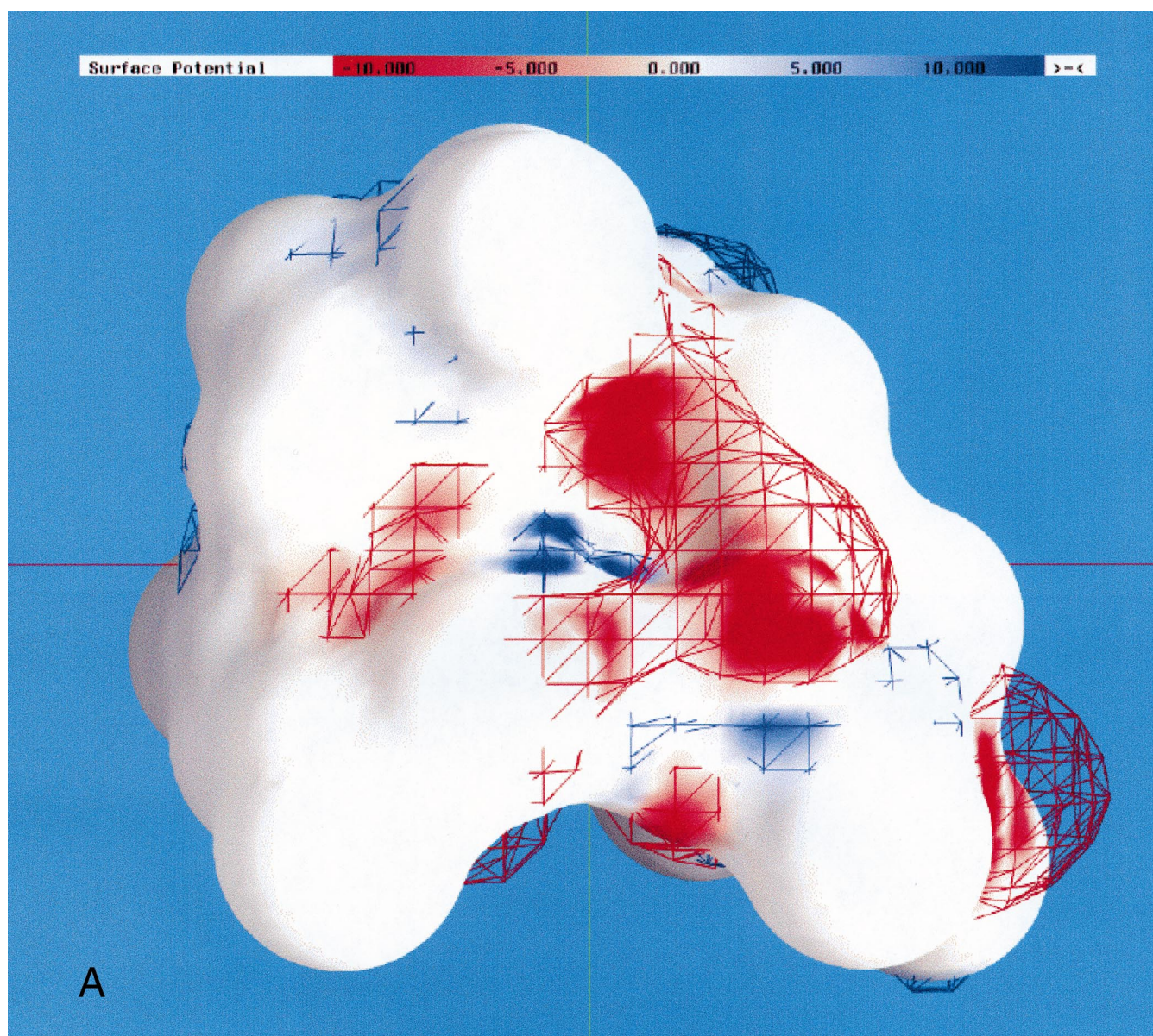
Fig. 4. Surface potential of the monensin complexes. (A) Mo-H, (B) Mo-Na and (C) Mo-K. Potentials more positive than +10\text{ kT/e} are deep-blue, potentials more negative than -10\text{ kT/e} are deep-red and neutral potentials ( 0\text{ kT/e} ) are white. 3D contours of the potential at +1 and -1\text{ kT/e} are shown in blue and red mesh. The level of polarity of each complex is reflected both in the ratio of colored vs. white region of the molecular surface and by the proximity of the contours to the molecular surface; polar complexes are characterized by large patches of red and blue on their molecular surface and by the fact that their contours are far from the molecular surface. It is obvious from the figure that Mo-K is significantly more polar than Mo-H and Mo-Na. The figure was generated by the GRASP program [38].
